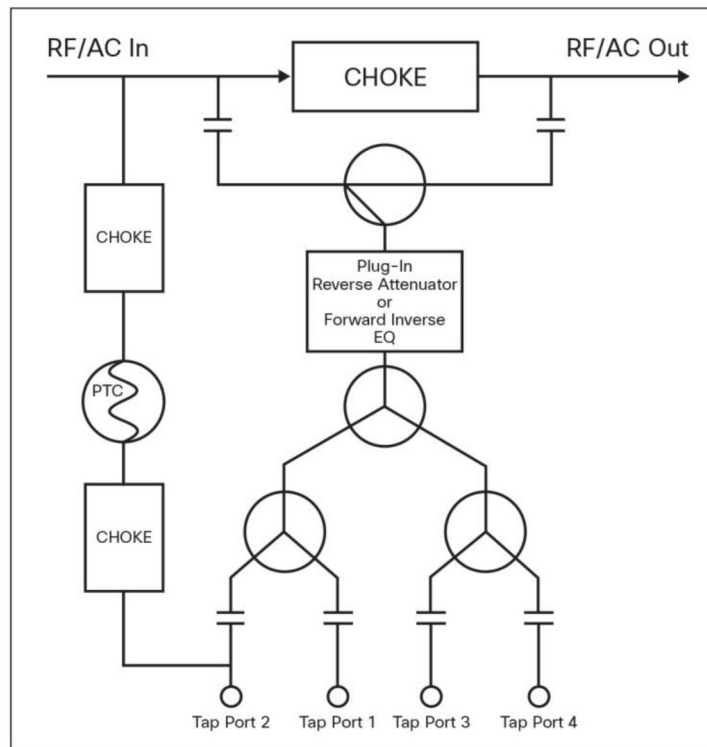
Functional Schematic
